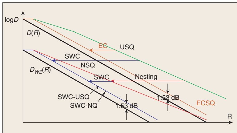
▲ 9. Performance of Gaussian Wyner-Ziv coding with scalar quantization and Slepian-Wolf coding.
